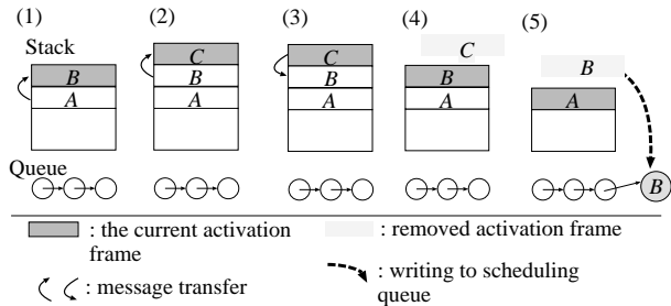
Figure 1: Intra-node scheduling strategy: (1) A sends a message to B . B starts execution immediately. (2) B sends a message to C . C starts execution immediately. (3) C sends the second message to B , and C continues execution because B is already active. (4) After C finished its execution, B executes the rest of the method. (5) When B finishes its method, B enqueues itself in the scheduling queue and will be scheduled later.
