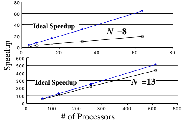
Figure 5: Speedup for N -queen problem ( N = 8, 13 ).
